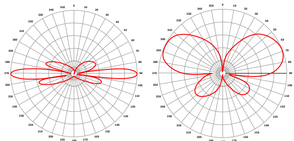
E Plane 896 MHz
